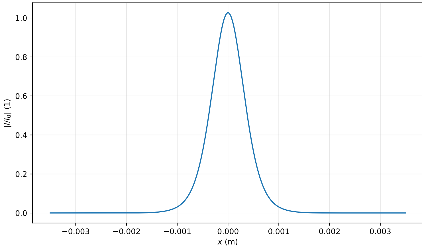
Intensity profile I(x, y = 0, z = 1.672m)/I_0 , P_{in}=0.6P_{cr} , artificial time
